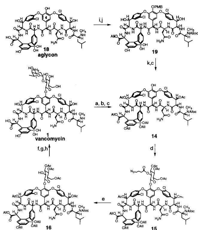
Scheme 3 a
