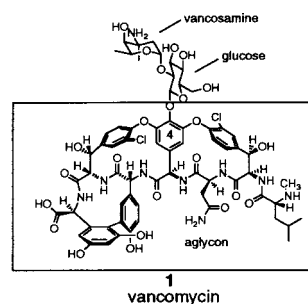
Figure 1. Glycopeptide antibiotic vancomycin.
